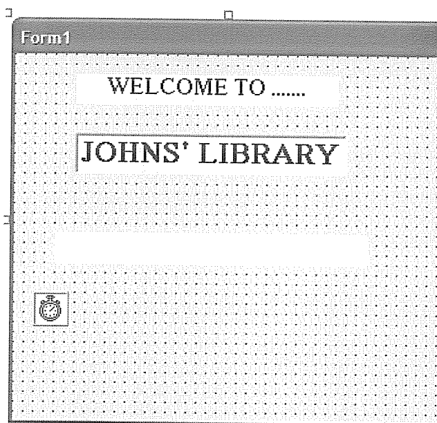
Figure 5: Splash screen
